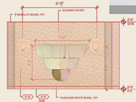
EAST LOBBY - ELEVATION N
