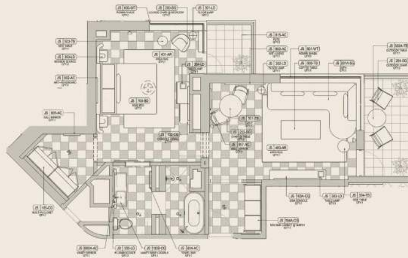
JUNIOR SUITE NORTH | FLOOR PLAN
